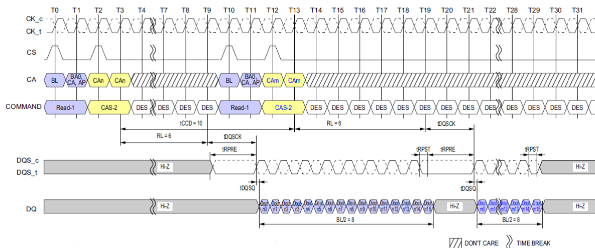
Figure 36. Consecutive Reads Operation: t_{\text{CCD}} = \text{Min} + 2 , Preamble = Static, 0.5nCK Postamble
