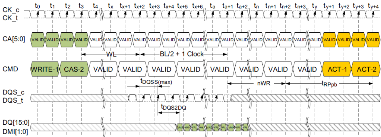
Figure 60. Burst WRITE with Auto-Precharge (Shown with BL16, 2tCK pre-amble)
