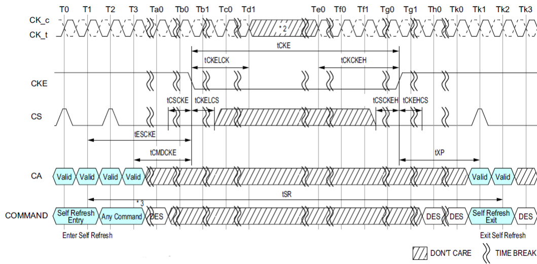
Figure 71. Self Refresh Entry/Exit Timing with Power Down Entry/Exit
