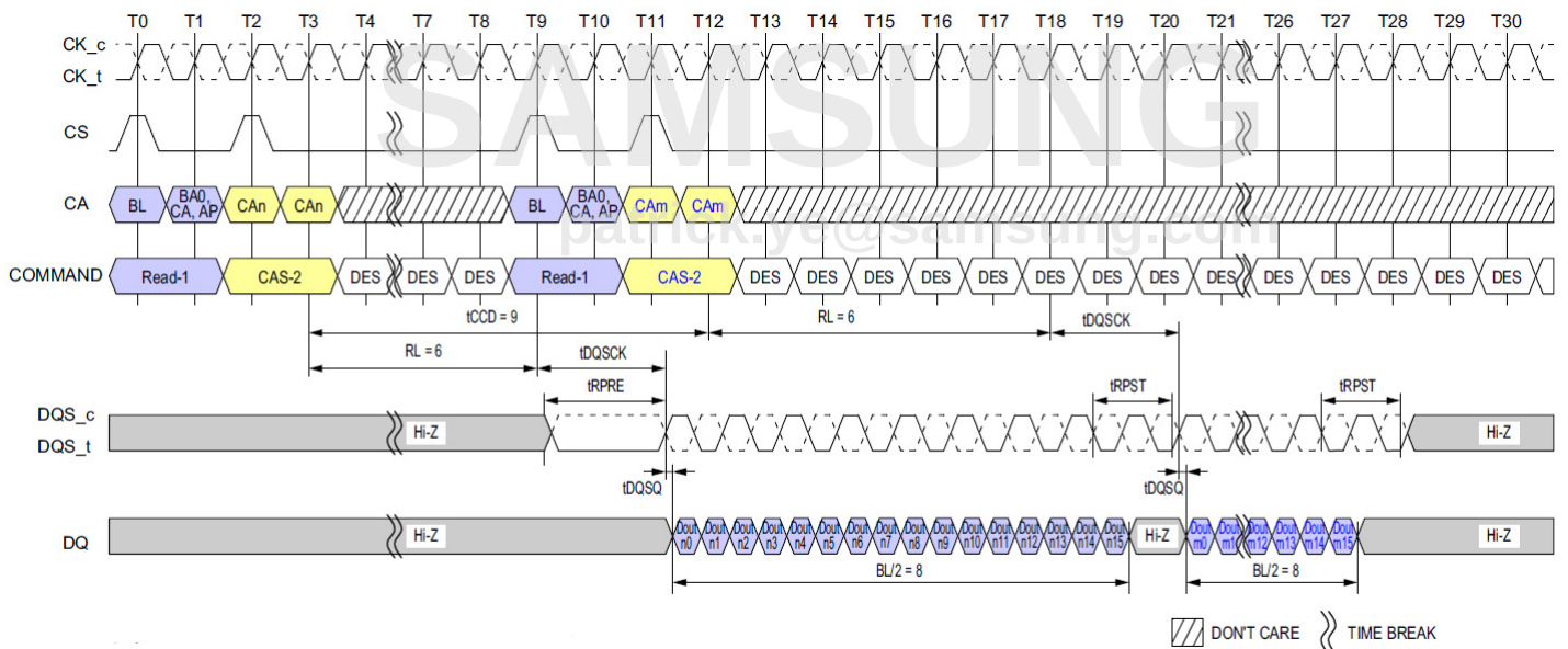
Figure 31. Consecutive Reads Operation: t_{CCD} = \text{Min} + 1 , Preamble = Static, 1.5nCK Postamble
