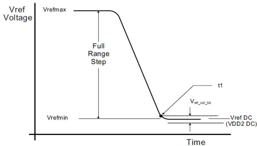
Figure 88. Vref full step from Vrefmax to Vrefmin case.
