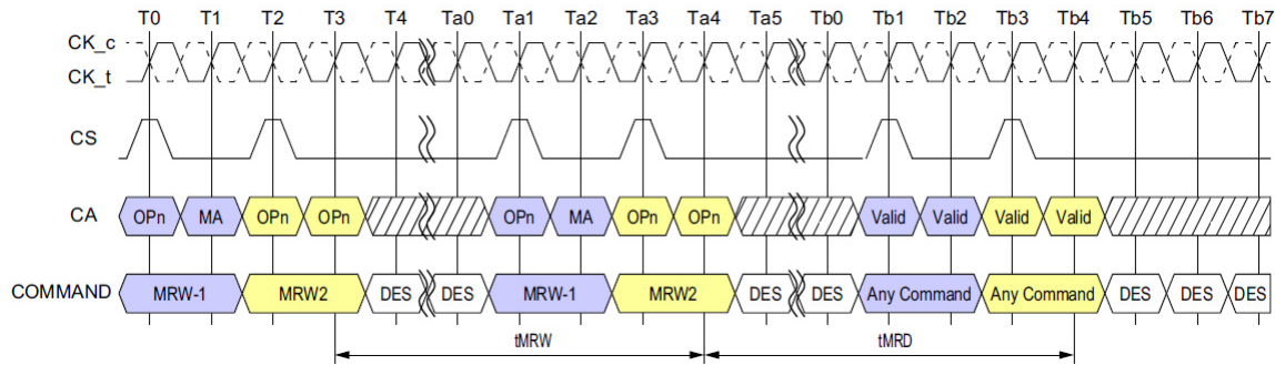
Figure 79. Mode Register Write Timing
