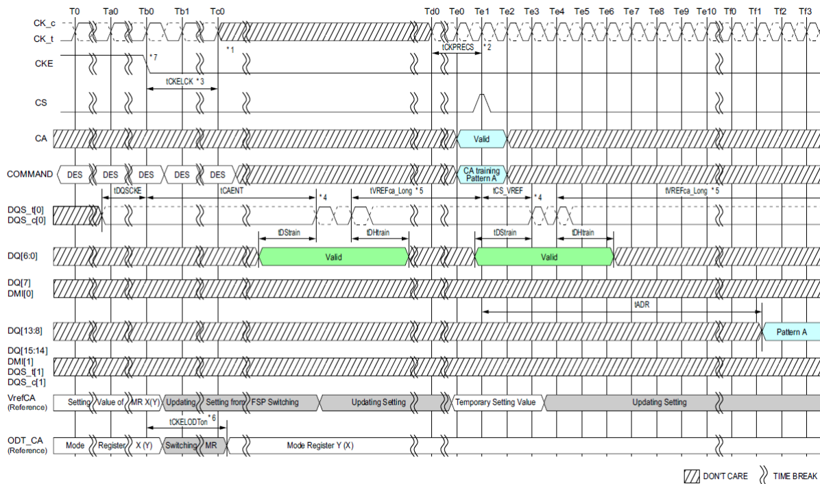
Figure 97. Consecutive V_{REFCA} Value Update
