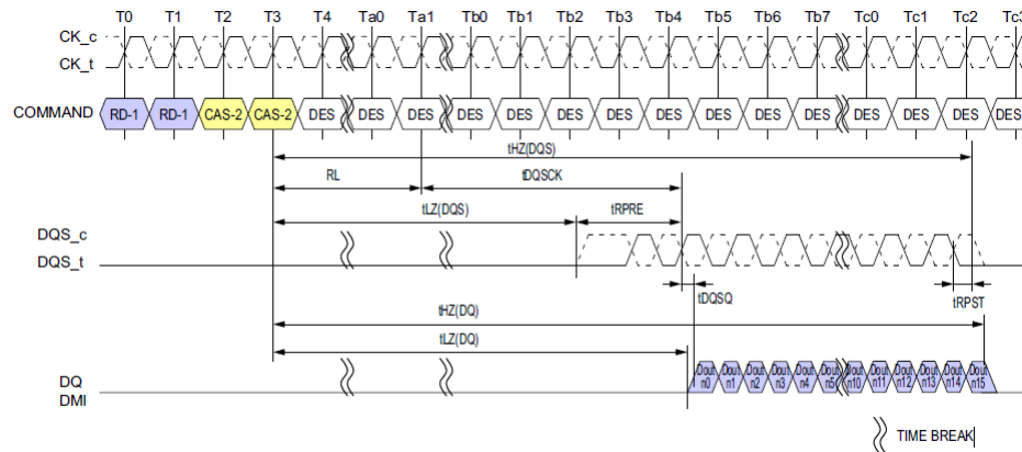
Figure 10. Read Timing
