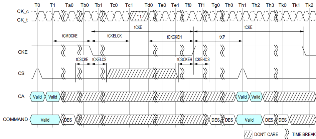
Figure 131. Basic power-down entry and exit timing
