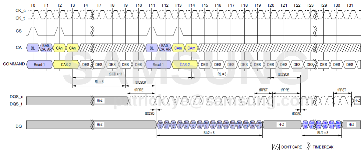
Figure 39. Consecutive Reads Operation: t_{CCD} = \text{Min} + 3 , Preamble = Static, 1.5nCK Postamble
