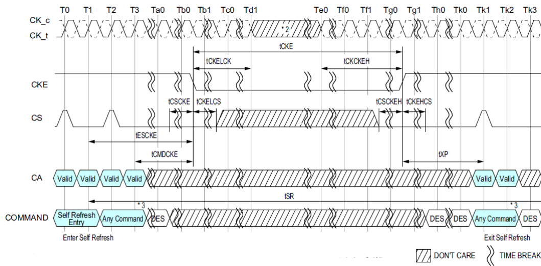
Figure 72. Command input timings after Power Down Exit during Self Refresh
