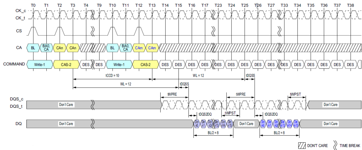
Figure 47. Consecutive Writes Operation: t_{CCD} = \text{Min} + 2, 1.5n\text{CK} Postamble
