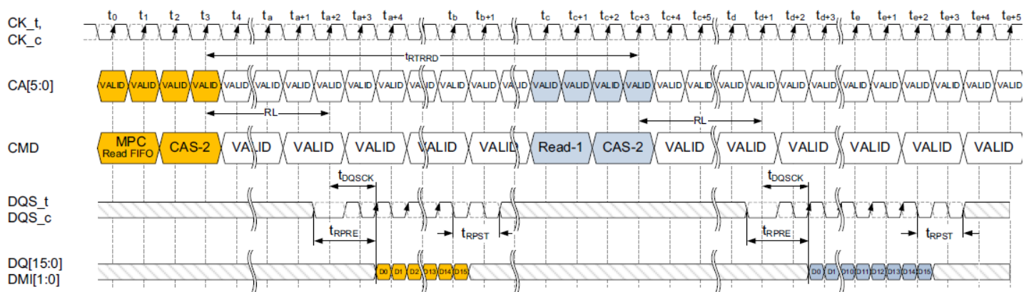
Figure 122. MPC [RD FIFO] Operation : tRPRE=toggling, tRPST=1.5nCK
