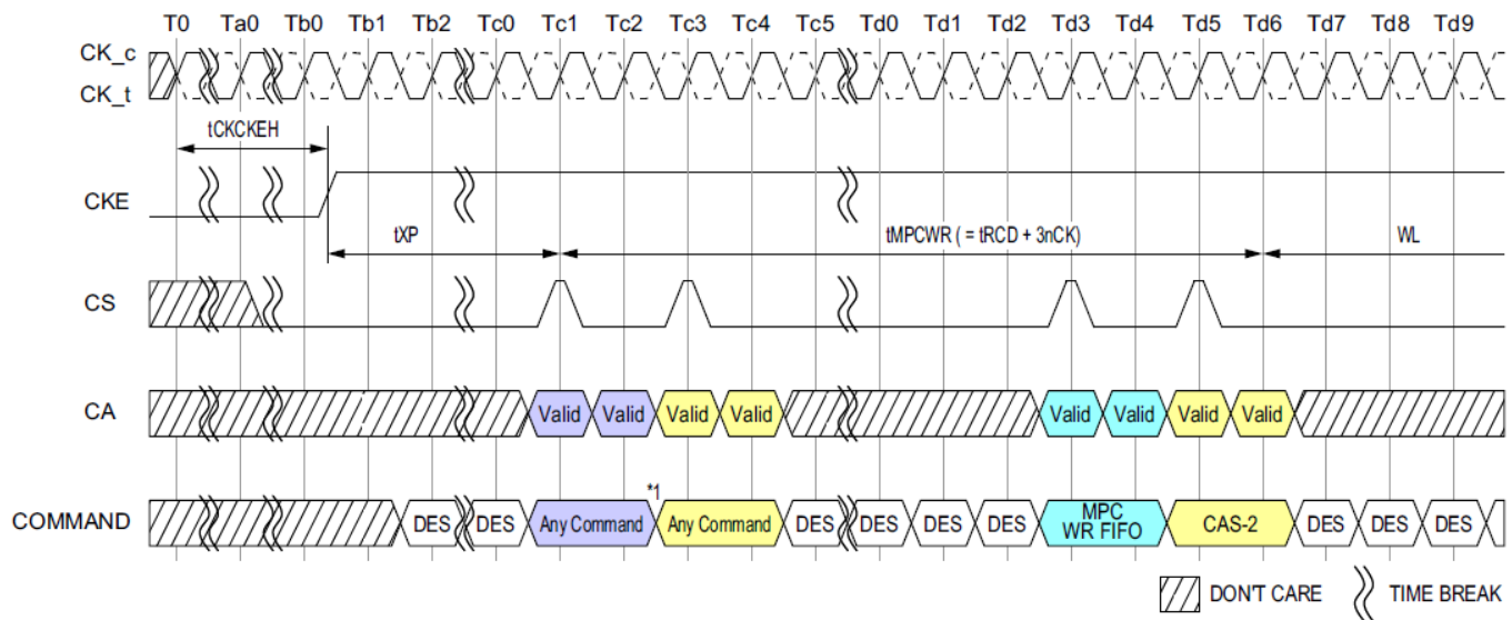
Figure 115. Power Down Exit to MPC [Write FIFO] Timing
