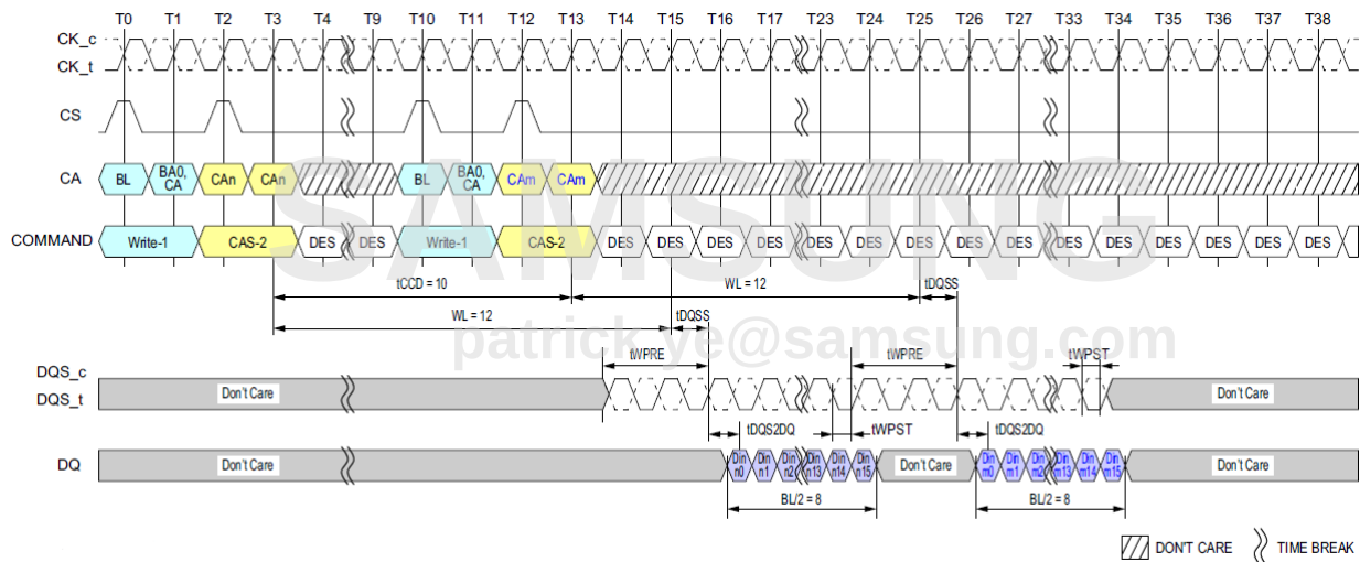
Figure 46. Consecutive Writes Operation: t_{\text{CCD}} = \text{Min} + 2, 0.5n\text{CK} Postamble
