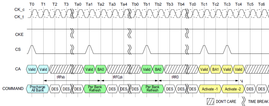
Figure 65. Per Bank Refresh to the same bank Operation
