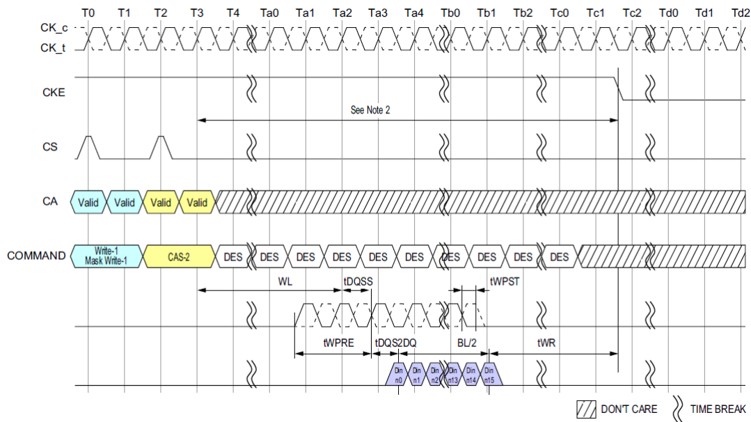
Figure 133. Write and Mask Write to Power-Down Entry
