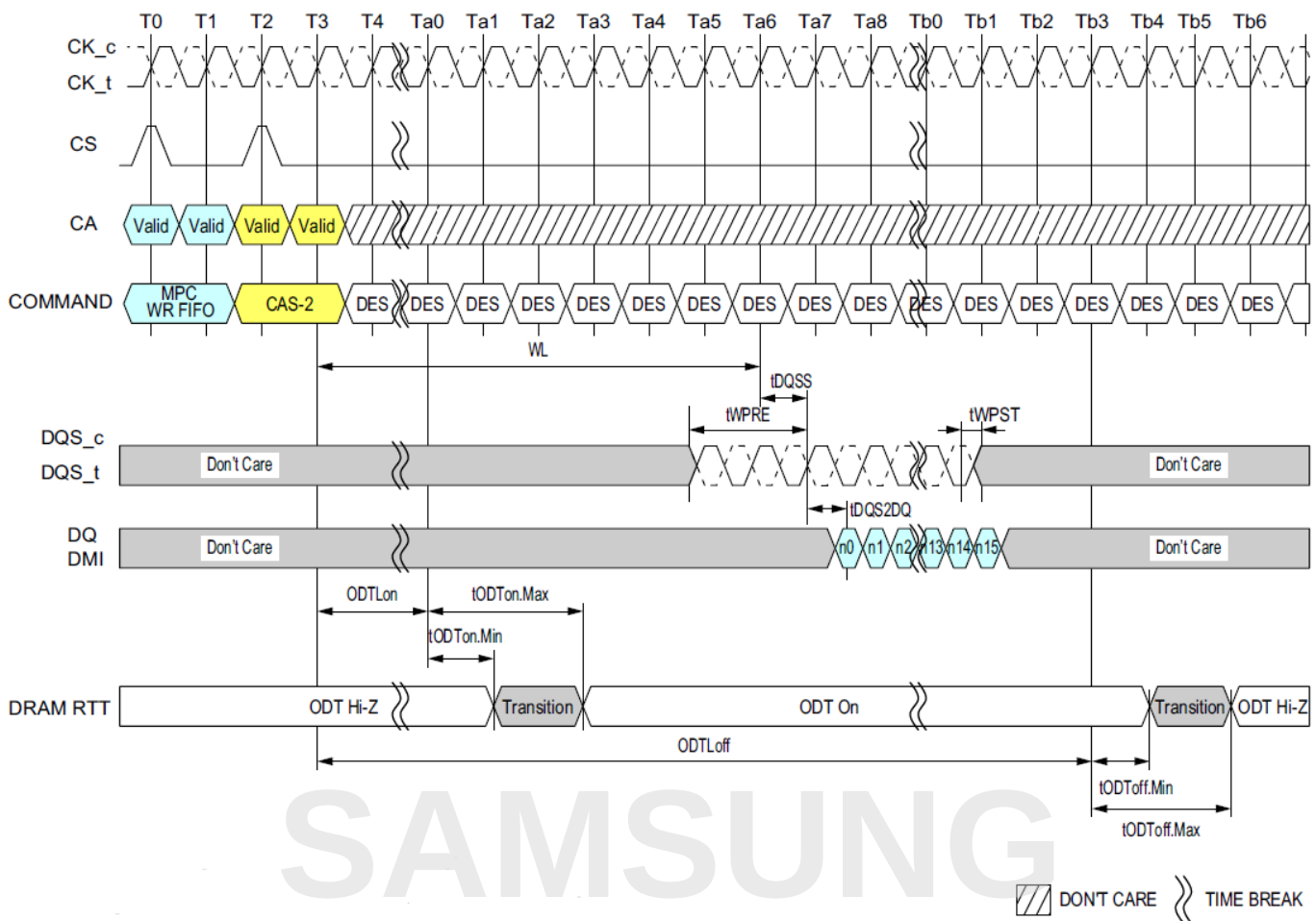
Figure 114. MPC [Write FIFO] with DQ ODT Timing
