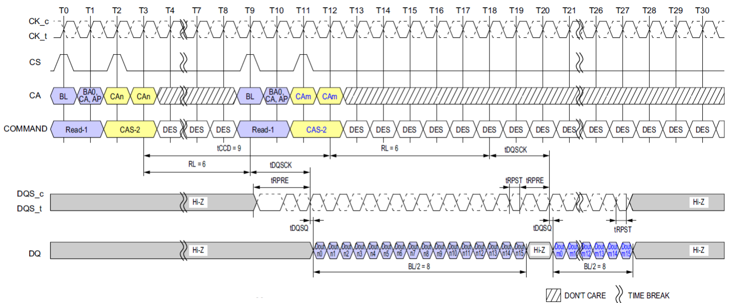
Figure 30. Consecutive Reads Operation: t_{CCD} = \text{Min} + 1 , Preamble = Toggle, 0.5nCK Postamble
