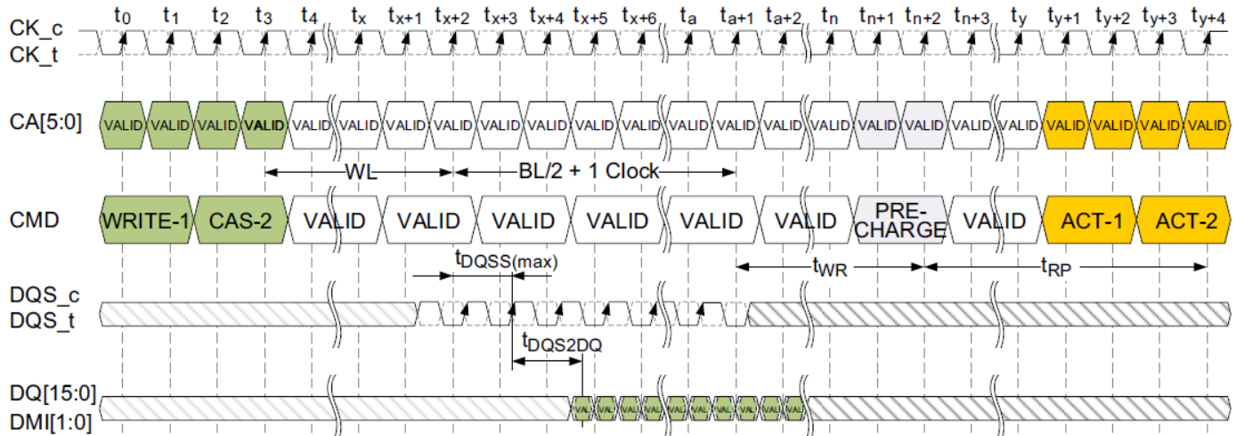
Figure 57. Burst WRITE Followed by PRECHARGE (Shown with BL16, 2tCK pre-amble)
