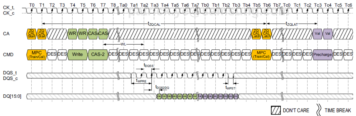
Figure 124. ZQCal Timing
