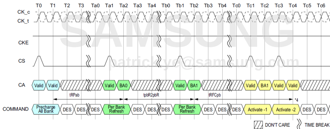
Figure 64. Per Bank Refresh to a different bank Operation
