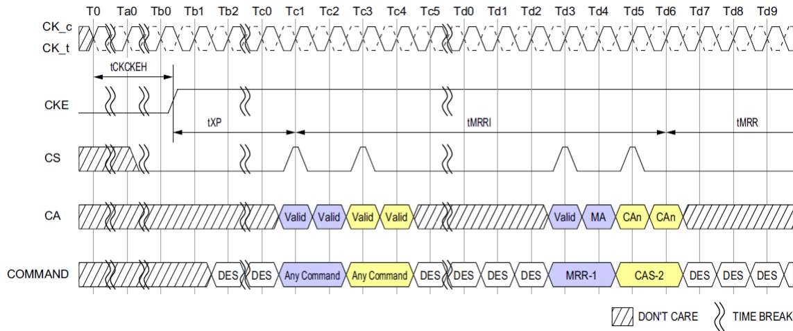
Figure 78. MRR Following Power-Down
