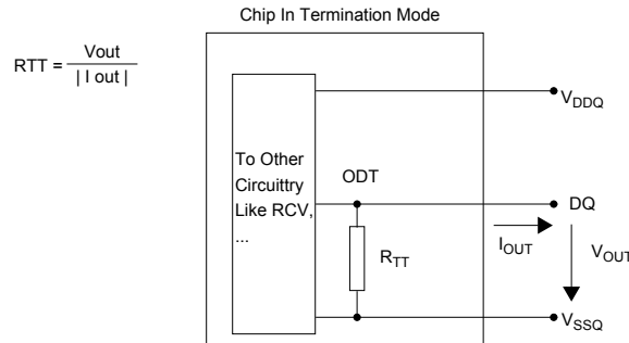
Figure 130. On Die Termination
