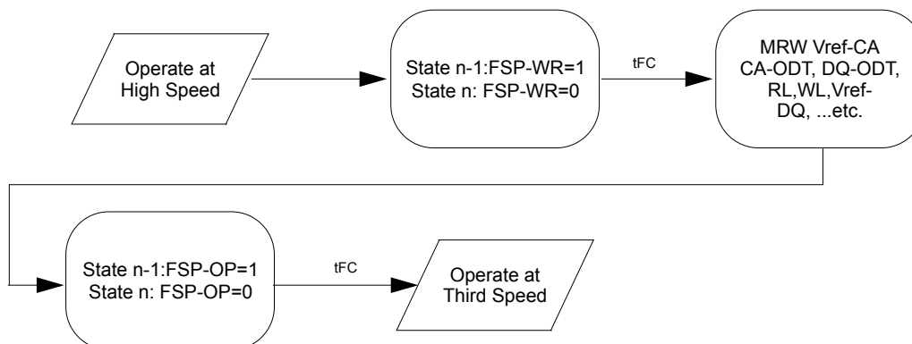
Figure 103. Switching to a Third Trained Frequency Set-Point
