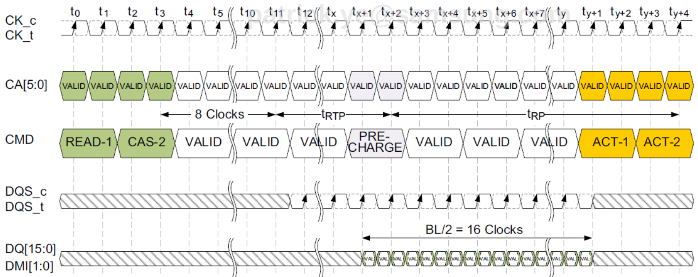
Figure 56. Burst READ followed by PRECHARGE (Shown with BL32, 2tCK pre-ample)
