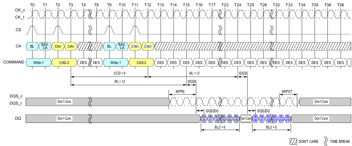
Figure 45. Consecutive Writes Operation: t_{CCD} = Min + 1, 1.5nCK Postamble
