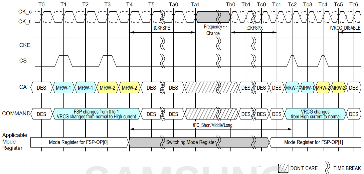
Figure 100. Frequency Set Point Switching Timing
