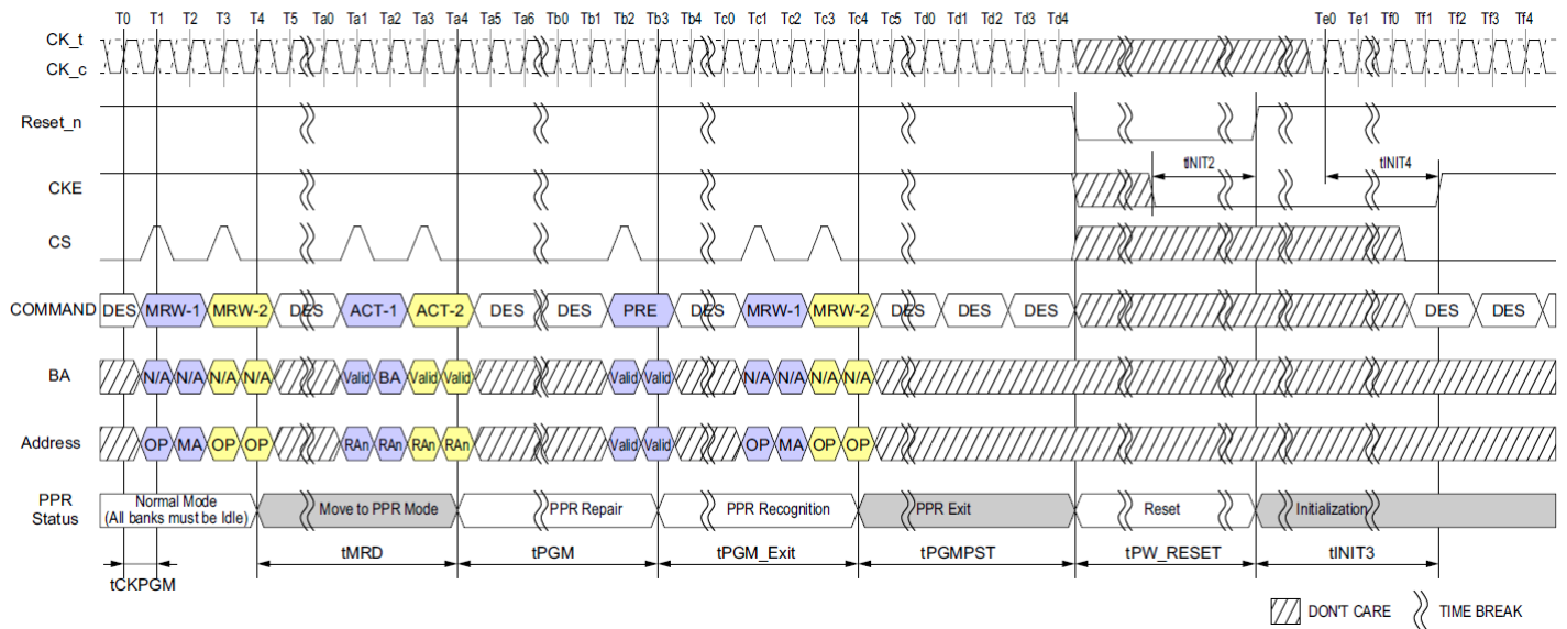
Figure 141. PPR Timing
