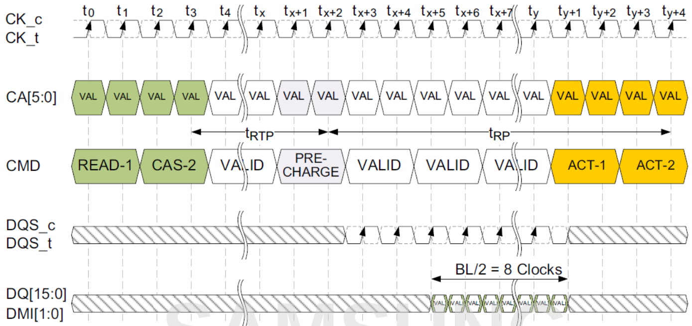
Figure 55. Burst READ Followed by PRECHARGE (Shown with BL16, 2tCK pre-ample)
