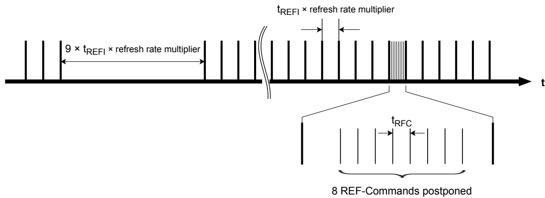
Figure 66. Postponing Refresh Commands (Example)
