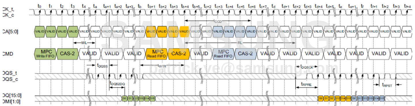
Figure 121. MPC [RD FIFO] Read Operation: t_{WPRE}=2nCK , t_{WPST}=0.5nCK , t_{RPRE}=toggling , t_{RPST}=1.5nCK
