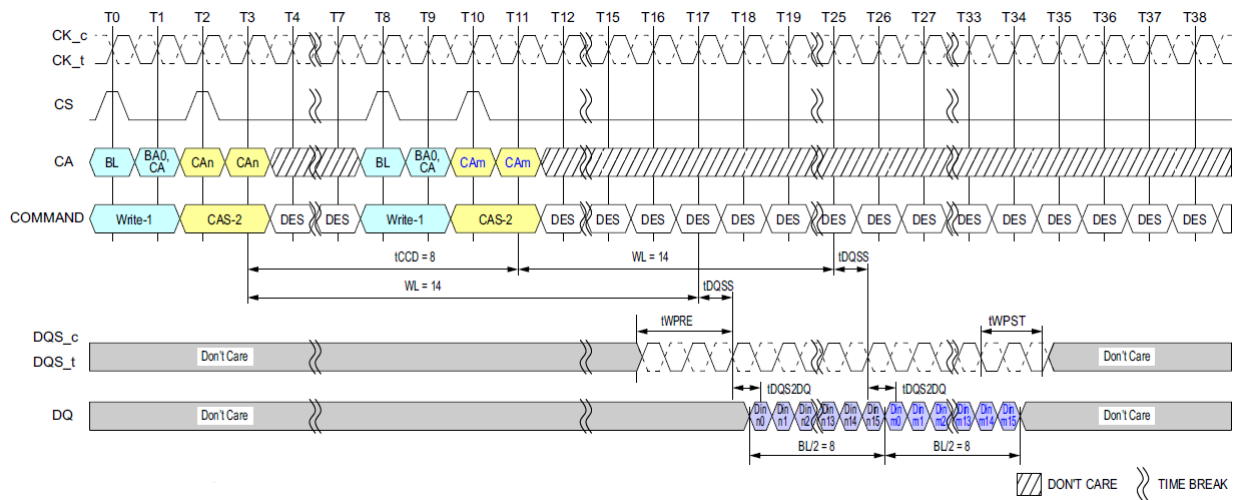
Figure 43. Seamless Writes Operation: t_{CCD} = \text{Min}, 1.5n\text{CK} Postamble
